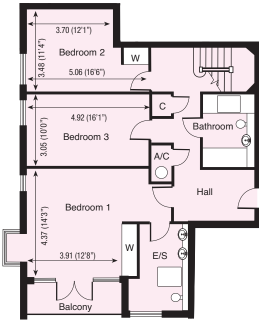
Lower Floor
