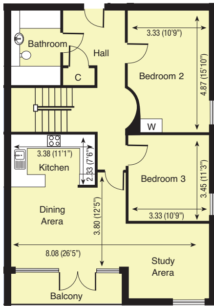
Lower Floor
